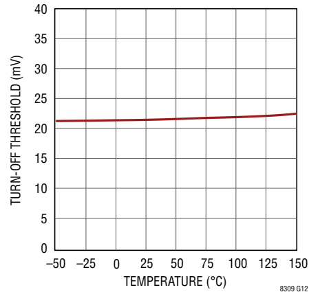
Comparator Turn-Off Threshold vs Temperature
