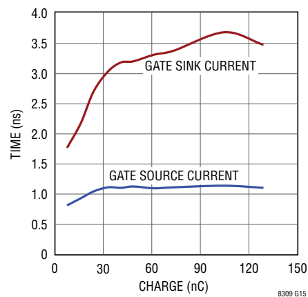
GATE Current vs Charge
